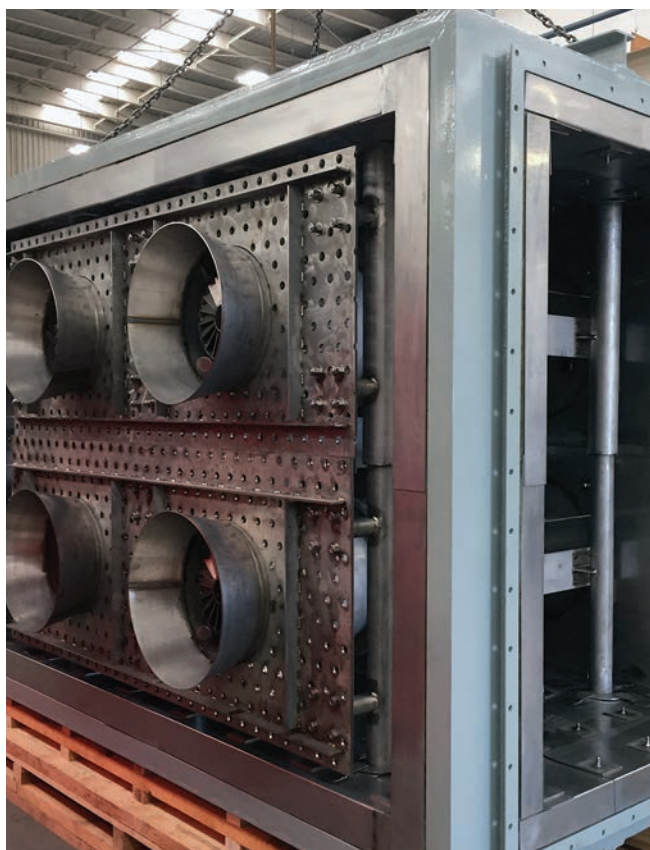
Register-Style Duct Burner
